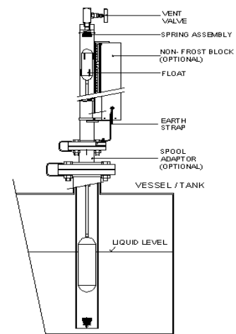
TOP MOUNT CONFIGURATION
